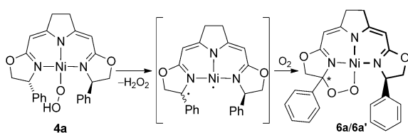
Scheme 5. Mechanistic proposal for the aerobic autoxidation of 4a .
